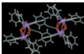
Fig. 2. Centrosymmetric dimers in the crystal structure of the title compound, formed by H23...O412 contacts ( cf. Table 1).
